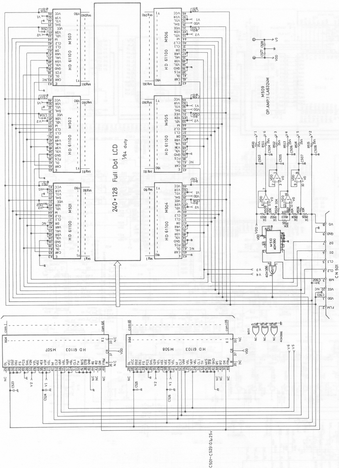
Figure 7-2. LCD PCB – Schematic Diagram
